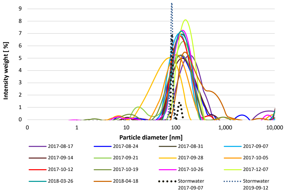
Figure S3. Particle size distribution intensity weight in washwater sampled by the street sweeping machine on 14 occasions, and in stormwater sampled on two occasions in the case study area. Analysed by dynamic light scattering (Litesizer TM 500).
