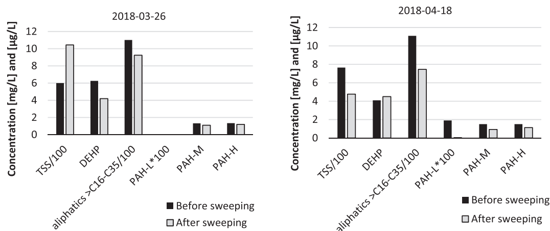
Fig. 6. The concentrations of TSS [mg/L] and OPs [ \mu\text{g/L} ] in WDS samples collected before and after street sweeping 2018-03-26 (left) and 2018-04-18 (right). Concentrations of OPs have been normalized towards the TSS concentrations in the samples.
