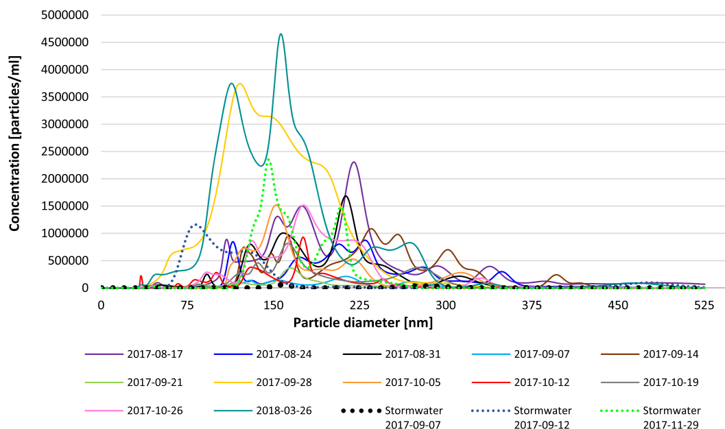
Fig. 3. Particle size distribution in wastewater sampled by the street sweeping machine on 12 occasions and in stormwater sampled on three occasions in the case study area. Analysed by nanoparticle tracking analysis (Nanosight).
