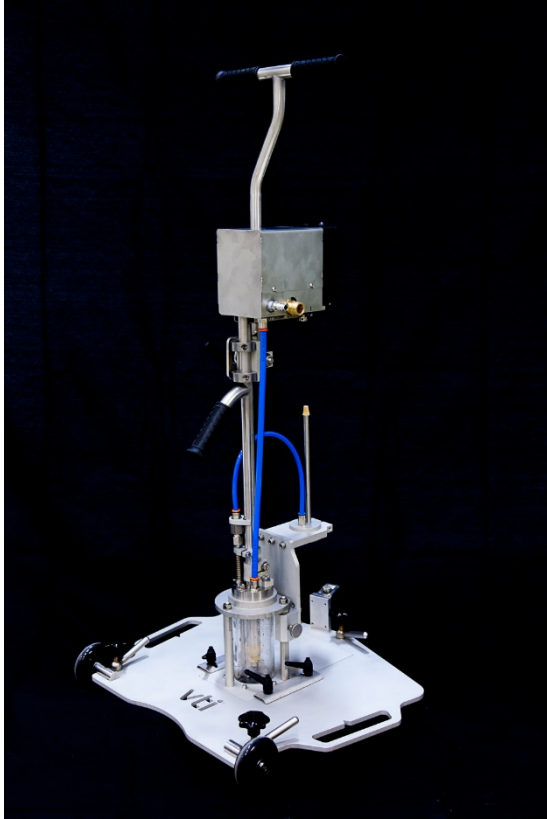
Figure S1. The VTI Wet Dust Sampler II (WDS II) used for sampling of road dust on road surfaces (photography: Mats Gustafsson, VTI).
