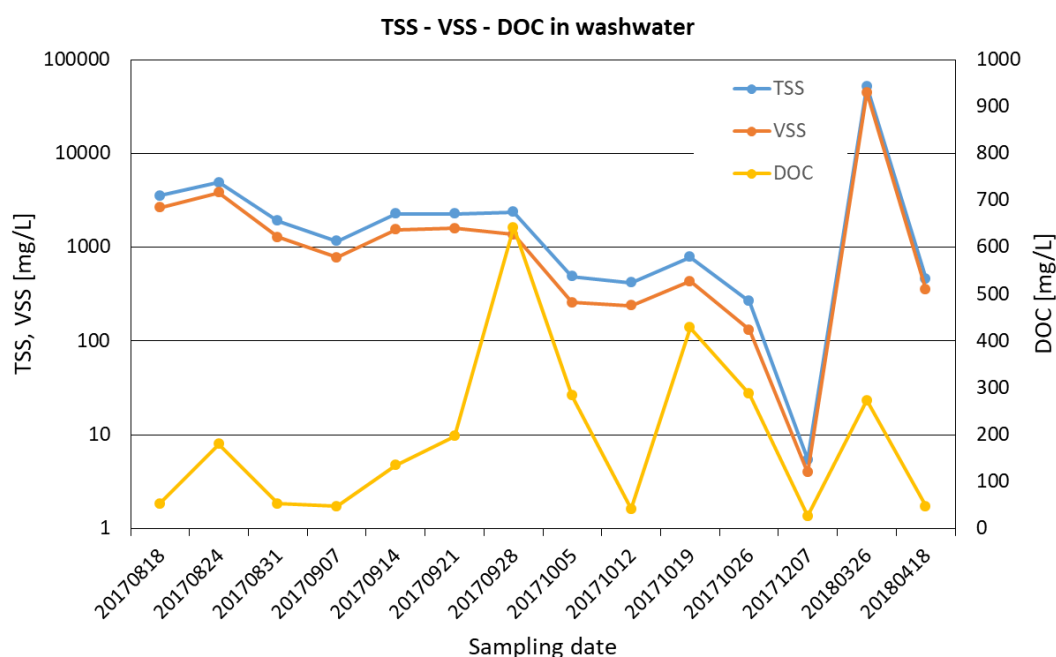
Figure S2. Concentrations of total suspended solids (TSS), volatile suspended solids (VSS) and dissolved organic carbon (DOC) in washwater samples.
